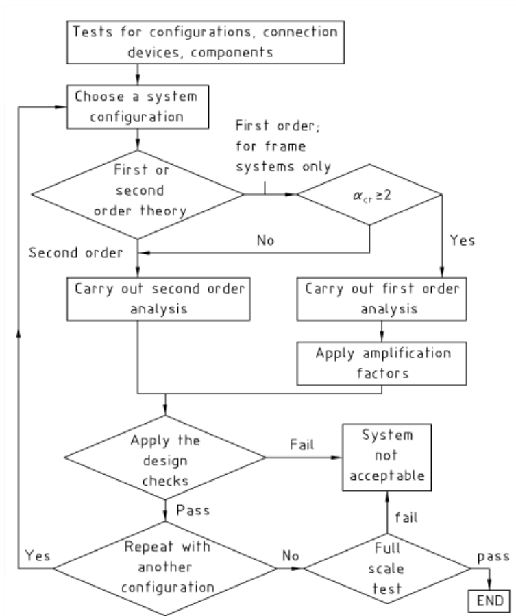
Figure 1 — Flow diagram of the stages of the structural design
